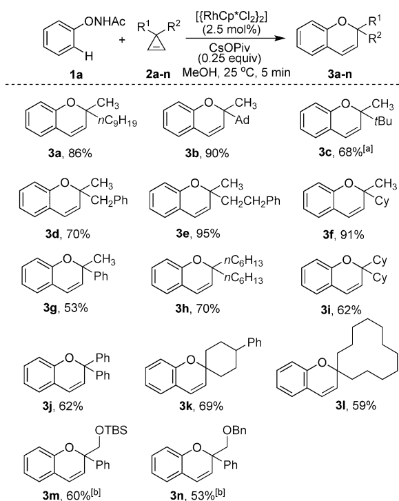
Scheme 2. Scope with respect to the cyclopropenes. If not otherwise noted, the reactions were carried out with 1a (0.20 mmol), 2a–n (0.26 mmol), [\{\text{RhCp}^*\text{Cl}_2\}_2] (2.5 mol %), and CsOPiv (0.25 equiv) in MeOH (4 mL) at 25 °C for 5 min under air. Yields are those of the products isolated after column chromatography. [a] Cyclopropene was added as a solution in pentane (0.3 M). [b] The reactions were carried out with 1a (0.36 mmol), 2m, n (0.20 mmol) at 25 °C for 10 min under air. Ad = adamantyl, TBS = tert -butyldimethylsilyl.
